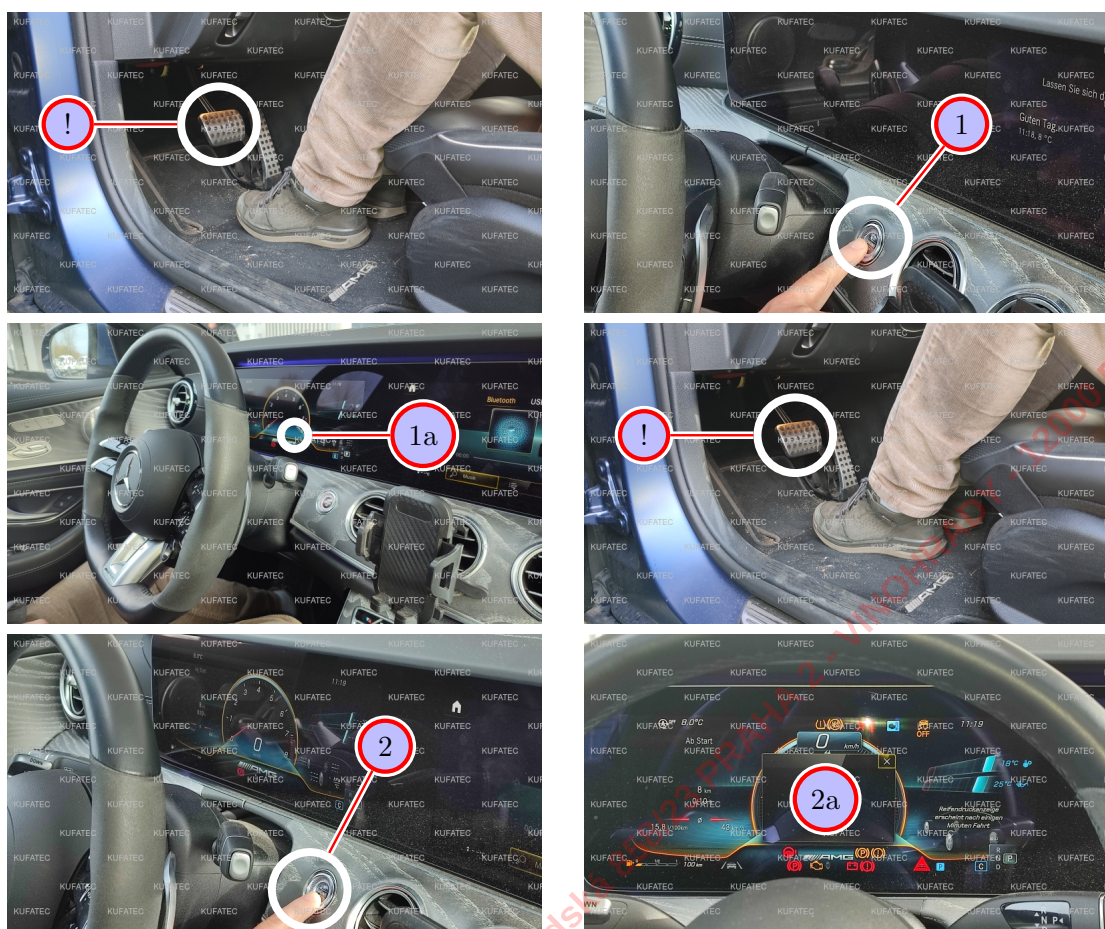
Figure 3: Ignition stage
